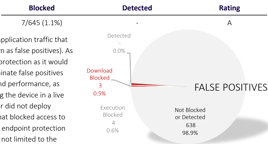
Figure 1 – False Positives
