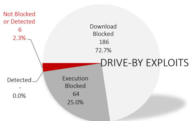
Figure 5 – Drive-by Exploits
