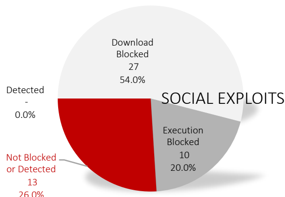
Figure 6 – Social Exploits
