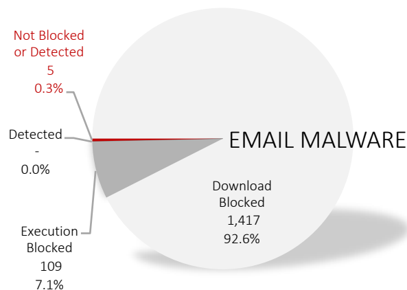
Figure 3 – Malware Delivered over Email
