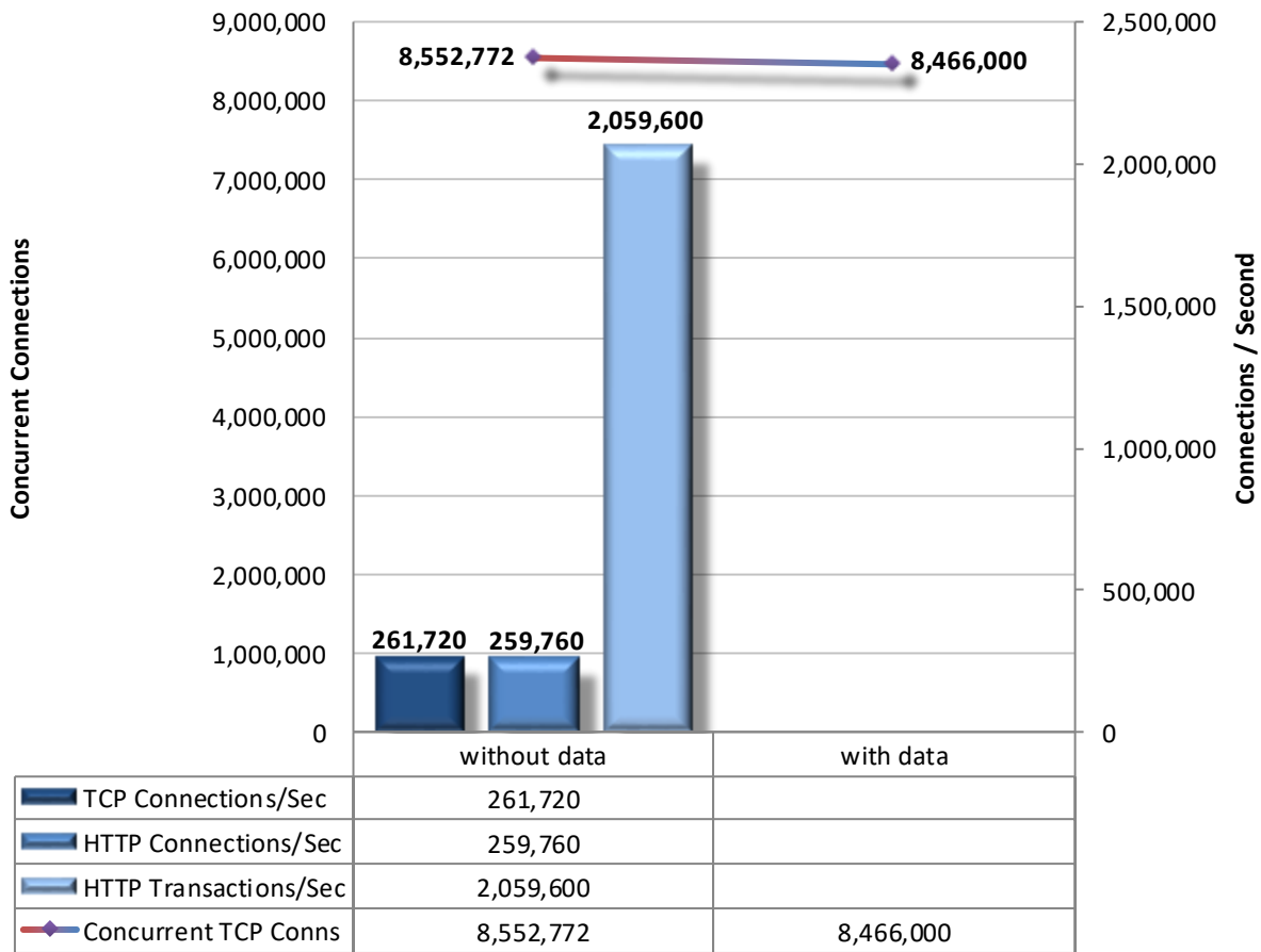
Figure 7 – Concurrency and Connection Rates (IPv6)
